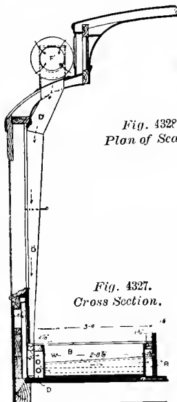
Fig. 4325-5. VENTILATOR FOR SALOONS.
